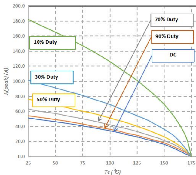
Fig.8-Current Derating
