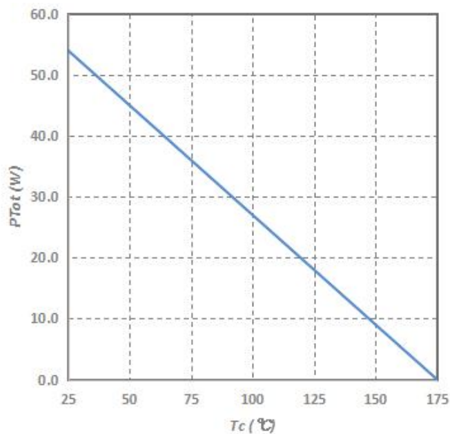
Fig.6-Power Derating
